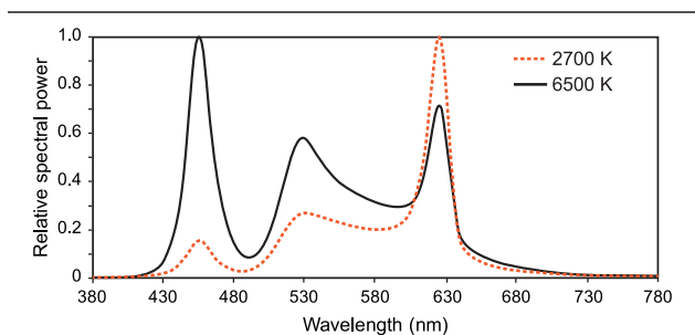
Figure 1. The spectral power distributions of the rated 2700 K and 6500 K LED white light sources used in the study.
