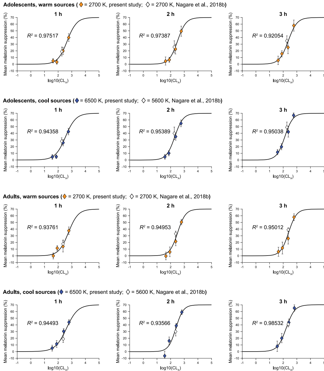
Figure 12. Using the least squares method, a 4-parameter logistic function (Rea et al., 2012) that converts CL_A to CS was used to best-fit the melatonin suppression data at each hourly exposure duration, by age group and light source. The warm sources include the 2700 K source from the present study (solid polygons) and a similar 2700 K source from a previous white light study (hollow polygons) (Nagare et al., 2018b). The cool sources include the 6500 K source from the present study (solid polygons) and a similar 5600 K source from the same, previous white light study (hollow polygons) (Nagare et al., 2018b). The error bars represent SEM. The threshold ( CS = 0.1 ) and half-saturation CL_A levels, derived using the respective best-fit plots, were subsequently converted to photopic light levels for the respective spectra, and are summarized in Table 4.
