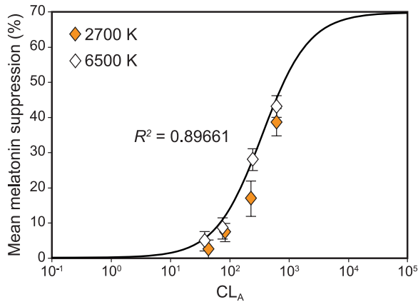
Figure 6. Logistic plot comparing the measured 1-h response data from the present experiment with the predicted responses from the original CS model to validate its accuracy. The data points correspond to mean nocturnal melatonin suppression following 1-h exposures to the 2700 K and the 6500 K sources at different corneal light levels ( CL_A , Equation 1). The continuous solid line represents the respective predicted CS values according to Equation 2 and depicts the functional relationship between CL_A and CS plotted without regard for the measured melatonin suppression values obtained in the present study. Goodness of fit ( R^2 ) for the logistic function is 0.90. The error bars represent SEM.
