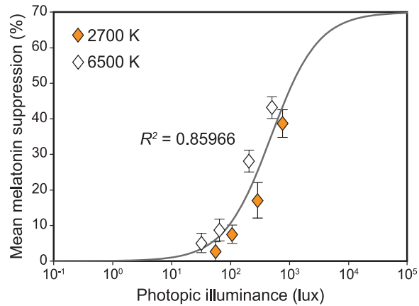
Figure 7. Logistic best-fit ( R^2 = 0.86 ) to the melatonin suppression data further plotted as a function of photopic illuminance levels, which is a widely used metric to characterize many human visual responses. For each target CS level, the higher photopic light levels for the 2700 K source consistently resulted in lower melatonin suppression compared with the circadian stimulus-matched 6500 K source providing lower photopic light levels. The error bars represent SEM.
