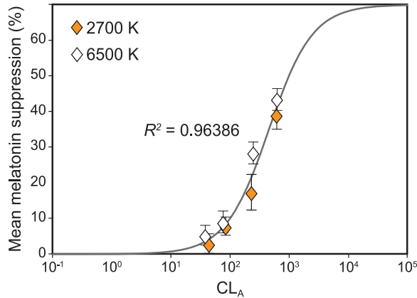
Figure 8. Logistic best-fit to the melatonin suppression data as a function of CL_A resulted in an improved fit ( R^2 = 0.96 ) while rectifying the discontinuity revealed by the fit as a function of photopic illuminance levels (see Figure 7). The error bars represent SEM. It is important to note that, while the original fit (see Figure 6) has been derived from the original Rea et al. CS model to validate its accuracy, the logistic best-fits as a function of the photopic illuminance levels (see Figure 7) and CL_A , shown here, are based on the formulation used by Zeitzer et al. (2000) and adapted from Rea et al., 2012 (Equation 4) to compare the effectiveness of the 2 metrics in characterizing the impact of light on nocturnal melatonin suppression (Rea et al., 2005; Rea et al., 2012; Rea and Figueiro, 2018).
